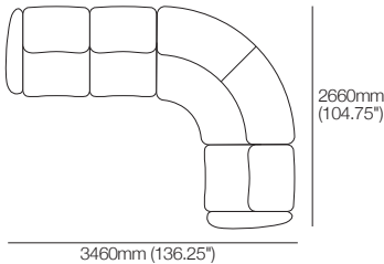
King Cinema 4-Seater with Corner Module | 4-Seater 800F
