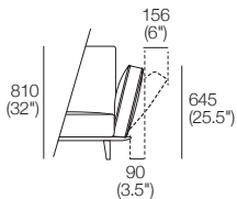
AB405 Closed + Recline Position Front View
