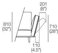
AB470 Closed + Recline Position Front View
