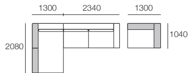
Package 1P
