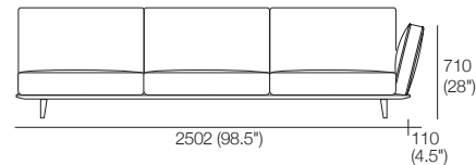
3 Seater 1 Arm P2502 (LH or RH) Components: 1x P2502, 3x C781, 3x AB570, 1x AB470
