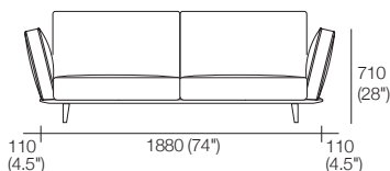
2 Seater P1880 Components: 1x P1880, 2x C781, 2x AB570, 2x AB470
