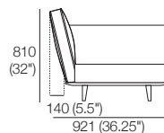
3 Seater 1 Arm P2502 (LH or RH) Side View
