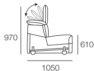
720R 720 FIXED Headrest 15 Levels
