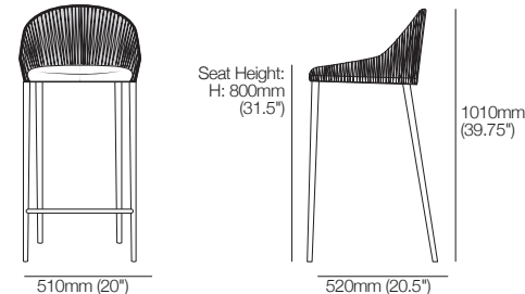
Barstool (WeatherWeave) Front View | Side View
