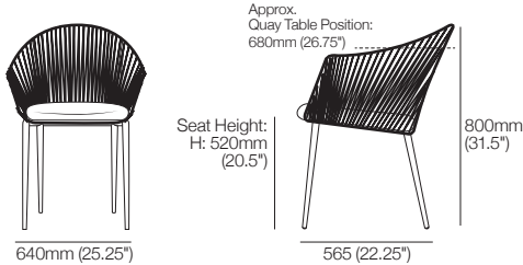
Dining Chair (Woven) Front View | Side View
