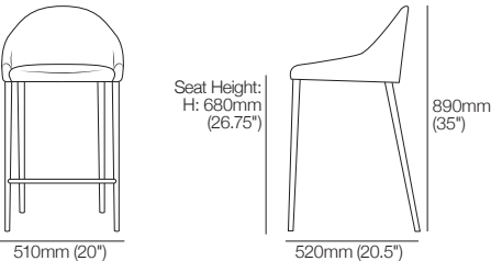
Counter Stool (Upholstered) Front View | Side View
