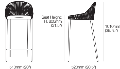
Barstool (Woven) Front View | Side View
