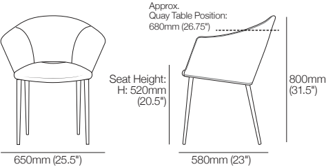
Dining Chair (Upholstered) Front View | Side View
