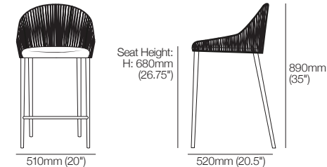
Counter Stool Woven) Front View | Side View
