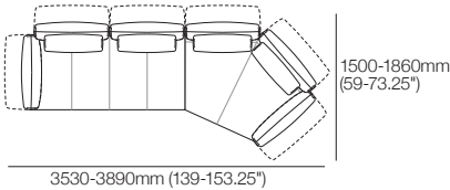
Haven Modular Sofa with Keystone Chaise 3530mm W Configurations: Right-hand | Left-hand Chaise
