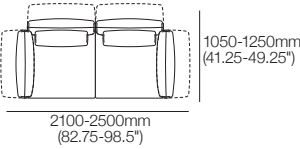
Haven Modular 2 Seater Sofa 2100mm W [2x 1-Seater Bases] Configurations:
